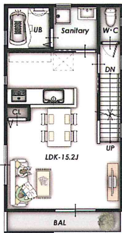
2F Plan
