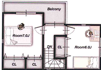
3Fplan
