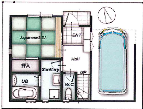
1Fplan
