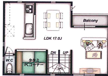
3Fplan
