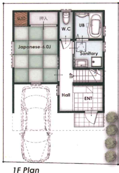
1F Plan
