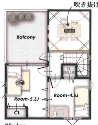
3Fplan
