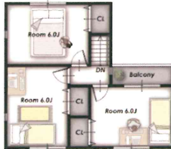
3Fplan
